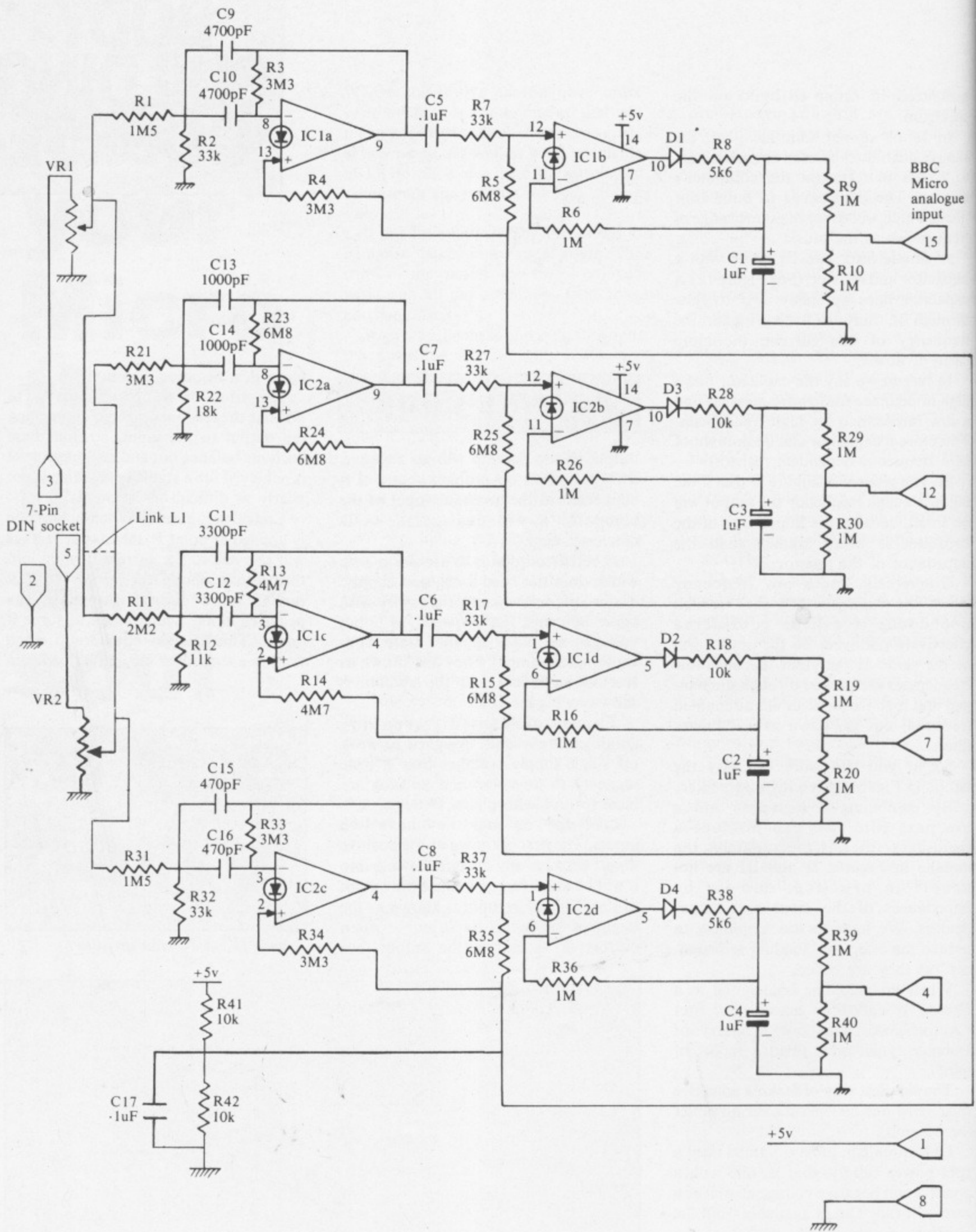
Figure VI: The sound-to-pattern converter
