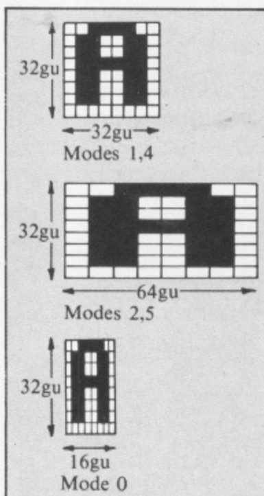
Figure IV. Character sizes in each graphic mode
