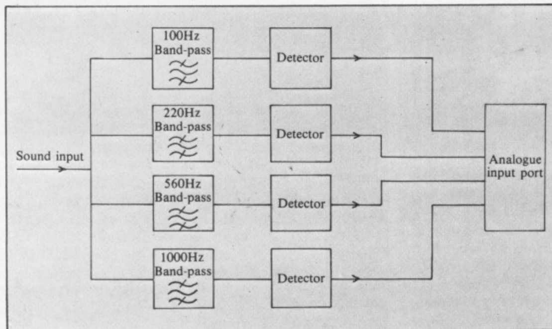
Figure I: Block diagram of our spectrum analyser
