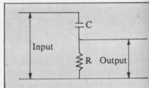
Figure III: A high pass filter
