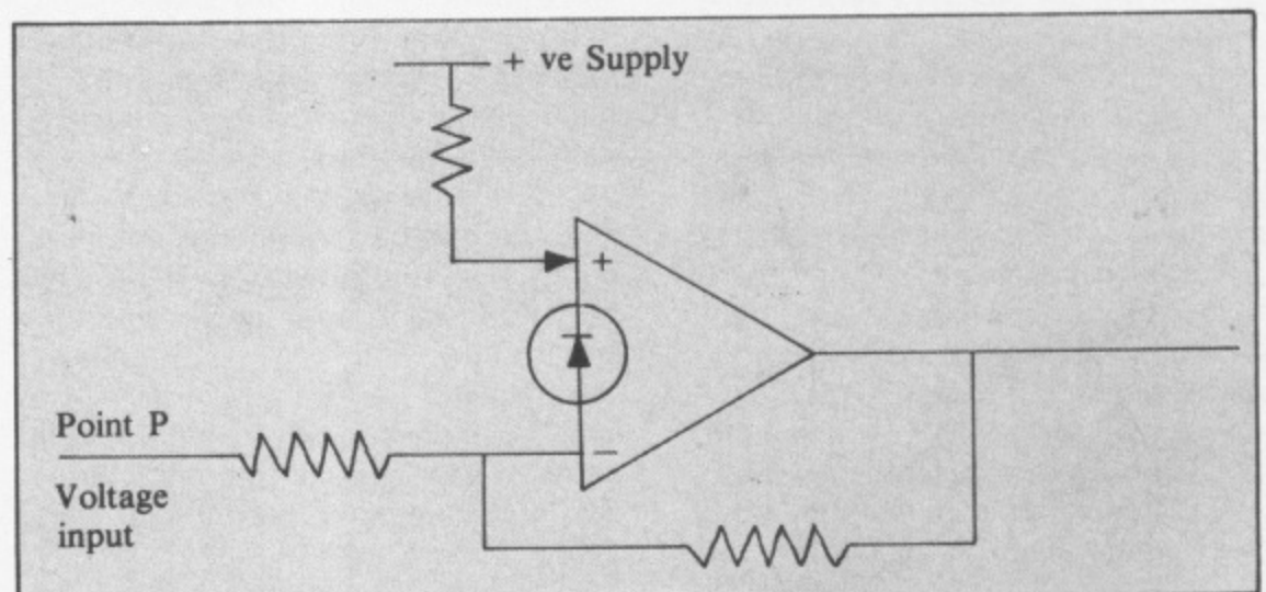
Figure V: An inverting amplifier
