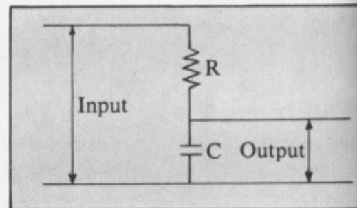
Figure II: A low pass filter
